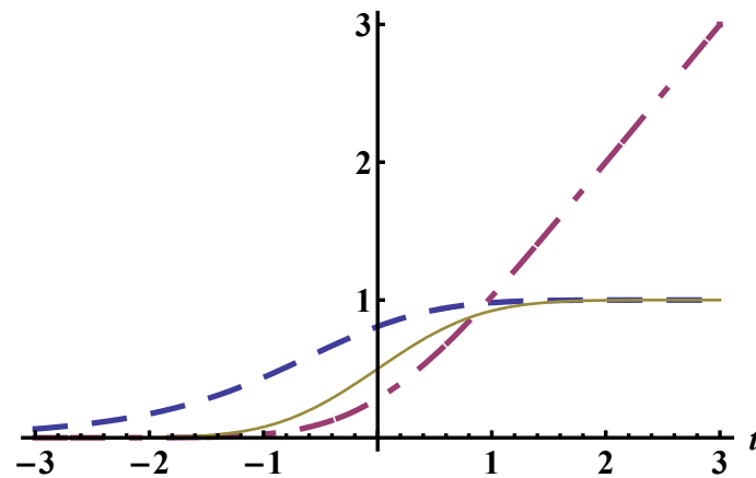
Fig. 1 The solid line is the force, the dashed line is V(t) , and dot-dashed is the solution V_0(t) (without radiation reaction), for \tau_0 = 1 = m .
