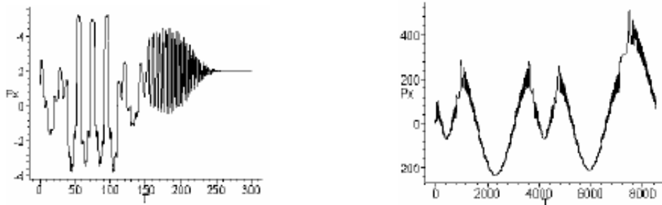
Fig.1 (P_x, T) Time series corresponding to the nonlinear equations of motion (a "flow" for H=0.9 ) A classical Fermi acceleration ("Chaotic or stochastic oscillations" along x- Axis) combined with the gun effect. Initial conditions (T, P_x, P_y, X) = (0.001, 1.5, 1.5, 0.001) .
