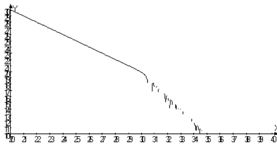
Fig.5.1. The plot of the function from (50) which can depicts the differential spectrum assigned to the synchrotron emission in arbitrary units
