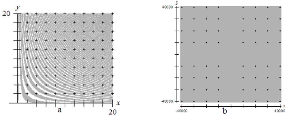
Fig. 3 The plot corresponding to the equation (34). The dashed domains are those where the inequality works; the x axis stands for \gamma^{-2} while the y axis stands for \frac{\langle \widehat{N} f^{(1)} / i \rangle_{k, \omega, 1}}{m_0^2 c^4} and \frac{\omega_{st}}{\omega} = 1 (a) and \frac{\omega_{st}}{\omega} = 10^3 (b)
