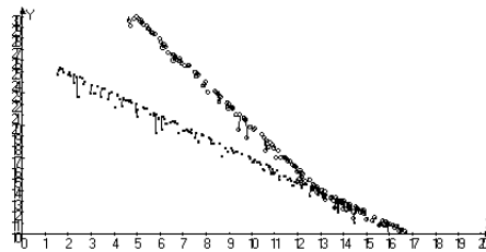
Fig.4.2. Two power spectra of the synchrotron emission for spectral indices of the number of particles \zeta = 7 (full squares) and \zeta = 9 (empty circles) . Y stands for \log P(\omega) and x stands for \log \omega ; both are in arbitrary units
