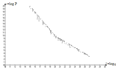
Fig.4.1 The power spectrum of the synchrotron emission derived in (44) where \log P is normalized to e^2 K_e (2\pi^2 c^3)^{-1} \tau^{-1} [0.5(m c^2)^2 + \langle Nf(1) \rangle]^{-1}
